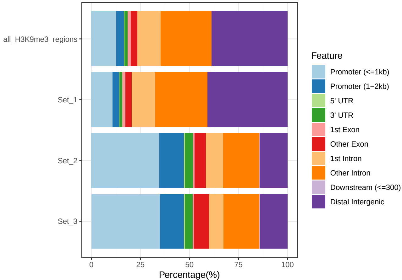
H3K9me3 Feature Distribution
